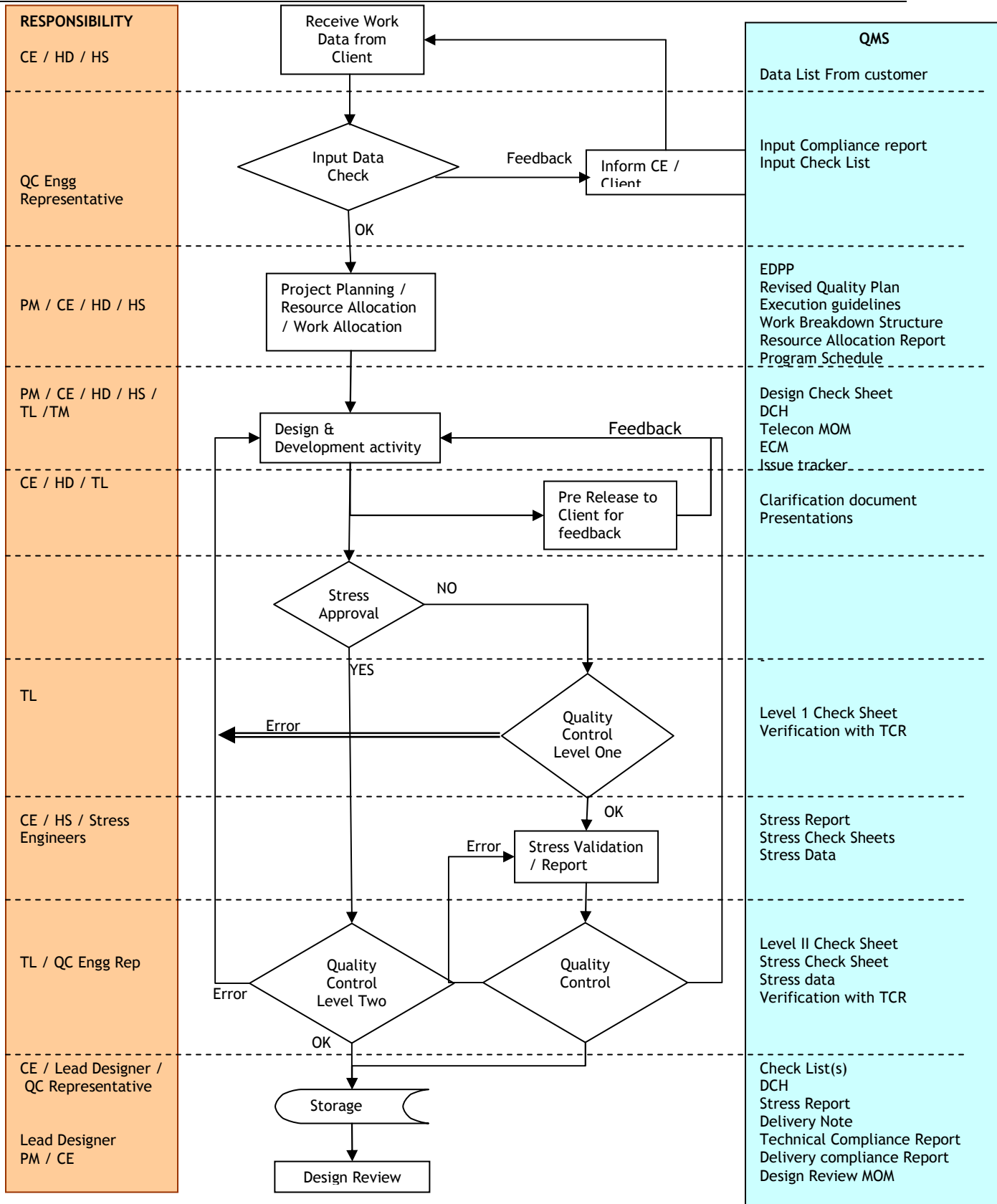
PROCESS FLOW
