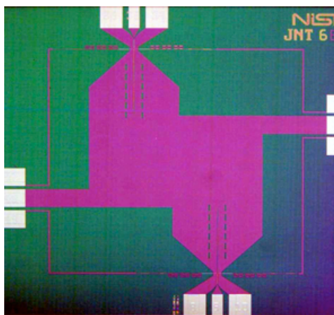
Photograph of circuit used in NIST's Johnson noise thermometry system. The system relies on the "noise" of jiggling electrons as a basis for measuring temperatures. It is extremely precise in part because it is based on the predictable quantum effects of superconducting elements located between the dashed slits on the top and bottom of the chip.
